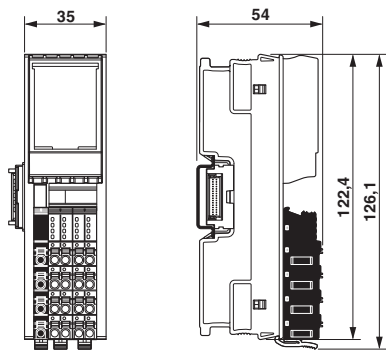
Dimensional drawing
