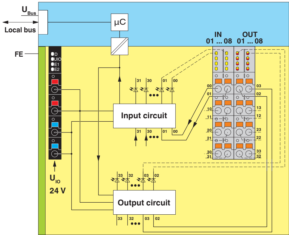
Block diagram
